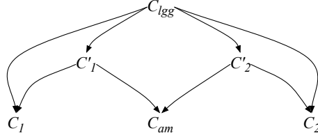
Fig. 1 A diagram of amalgamation from descriptions C_1 and C_2 with an amalgam C_{am} . Arrows indicate the subsumption of the target by the source of the arrow.
